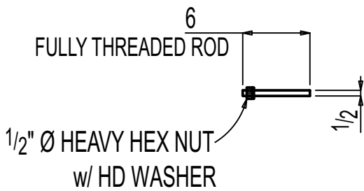
2 THREADED RODS F-12.03M1
